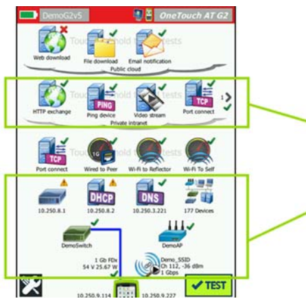
Figure 1. The AutoTest provides a comprehensive measurement of network performance from the end user point-of-view, from cable, to services and applications (Test result from OneTouch AT with G2 Modules for both Wired and Wi-Fi network shown)
