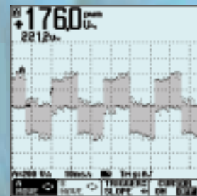
V_{pwm} measures effective voltage on motor drive and frequency inverter outputs.
