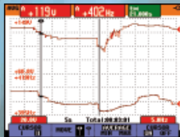
Cursors and zoom function help you to analyze the captured TrendPlot.
